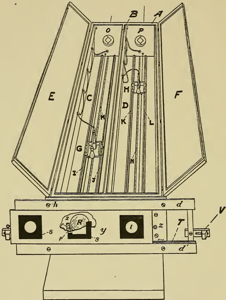
FIG. 6. PERSPECTIVE OF LIGHT OR "BRIGHTNESS" APPARATUS
